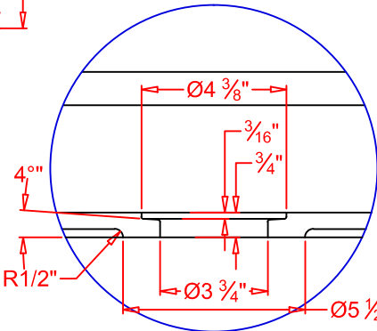
DRAIN DETAIL
