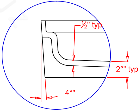
WALL / PANEL PLATFORM DETAIL
