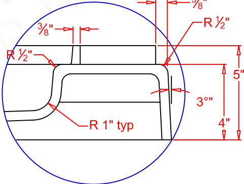
THRESHOLD DETAIL
