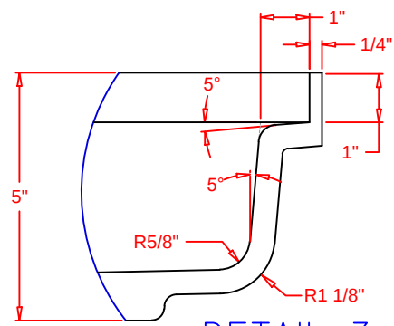
DETAIL 3
