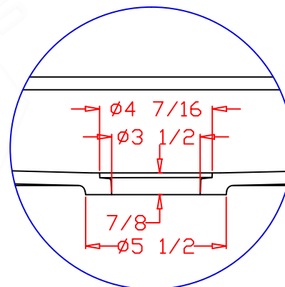
Detail 1 Drain Section
